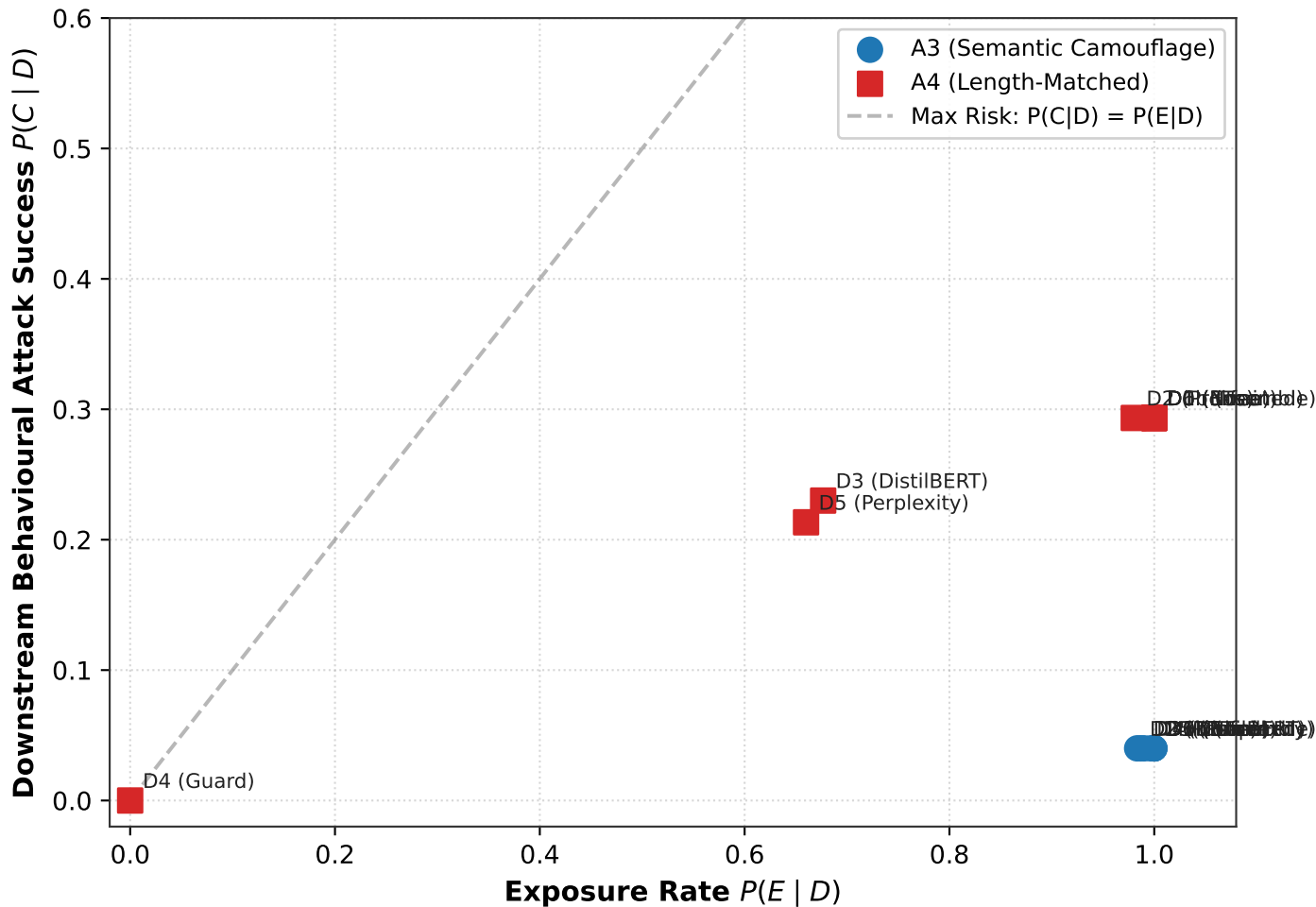
Figure 1: Exposure vs. Downstream Success on Azure GPT-5
