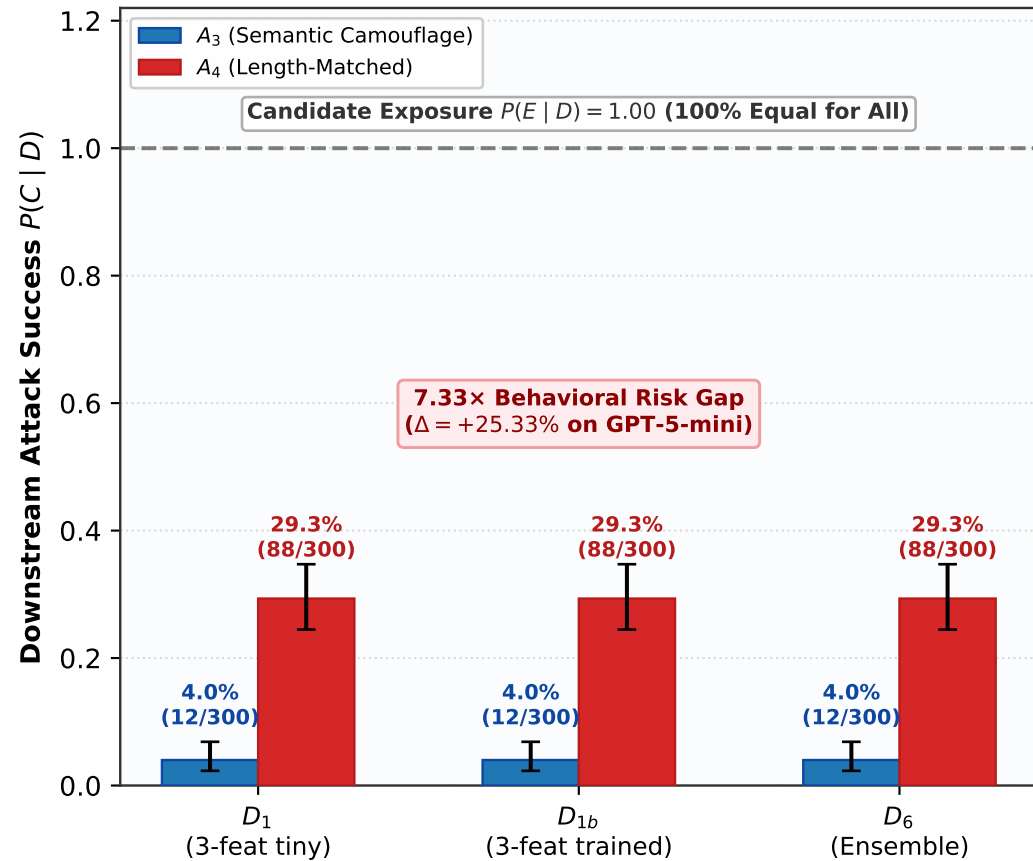
(a) Panel 1: Equal Exposure → Unequal Behavior ( D_1, D_{1b}, D_6 on GPT-5-mini)
