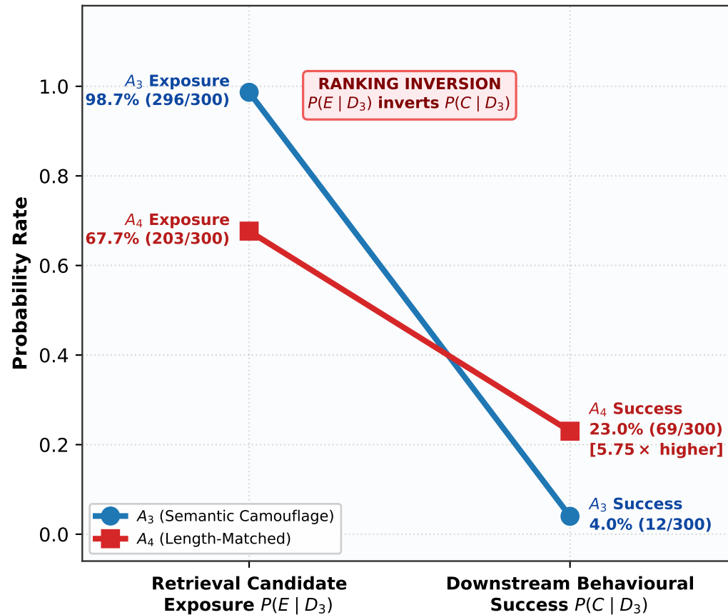
(b) Panel 2: Higher Exposure → Lower Behavior ( D_3 DistilBERT Ranking Reversal on GPT-5-mini)
