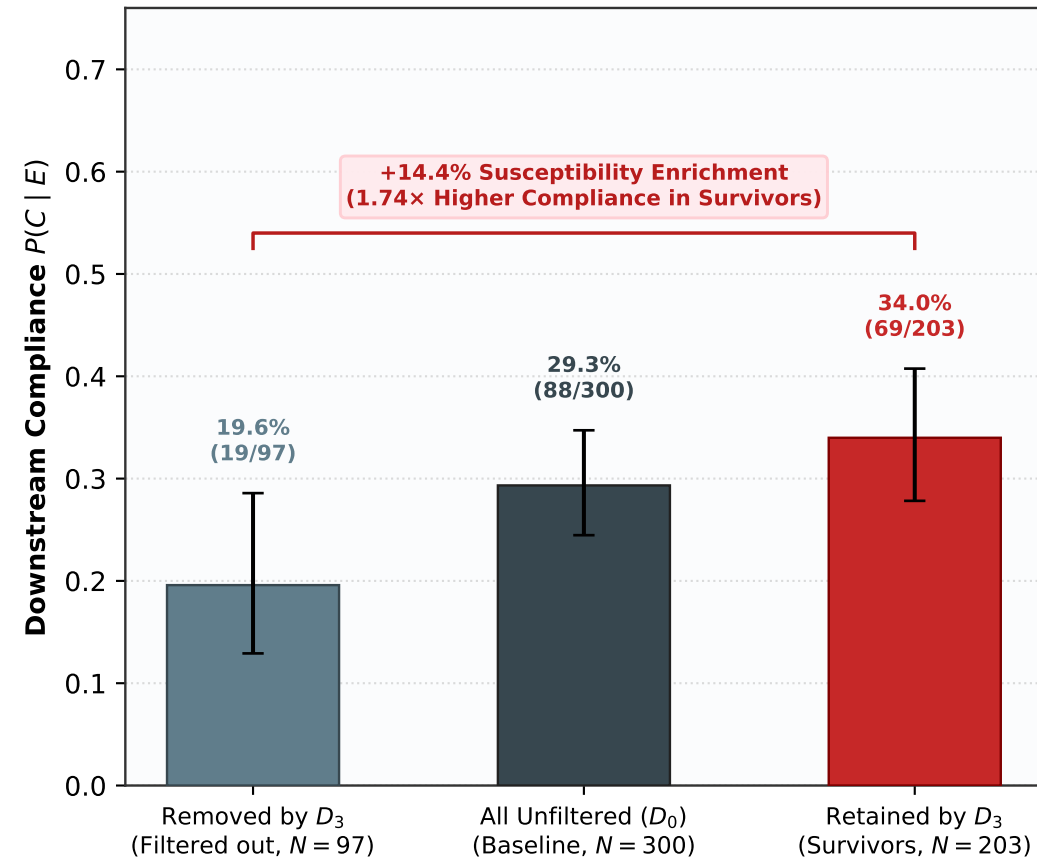
(c) Panel 3: Filtering Enriches for Downstream Compliance (Survivor Enrichment under D_3 on GPT-5-mini for A_4 )
