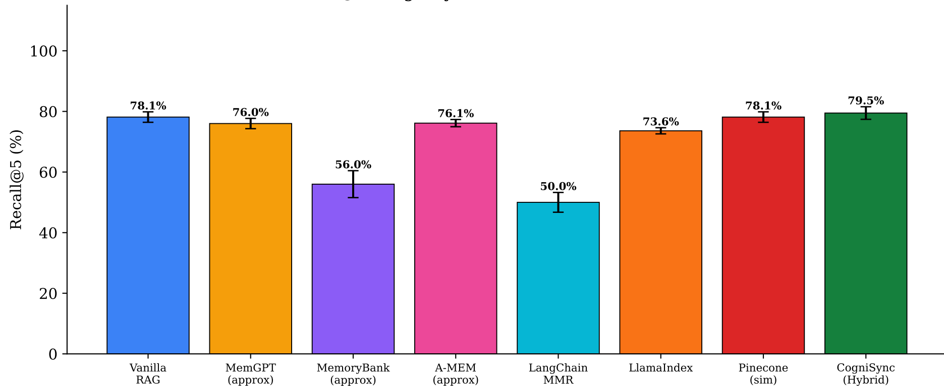
Retrieval Recall@5: CogniSync vs All Baselines (5-trial mean +/- std)
