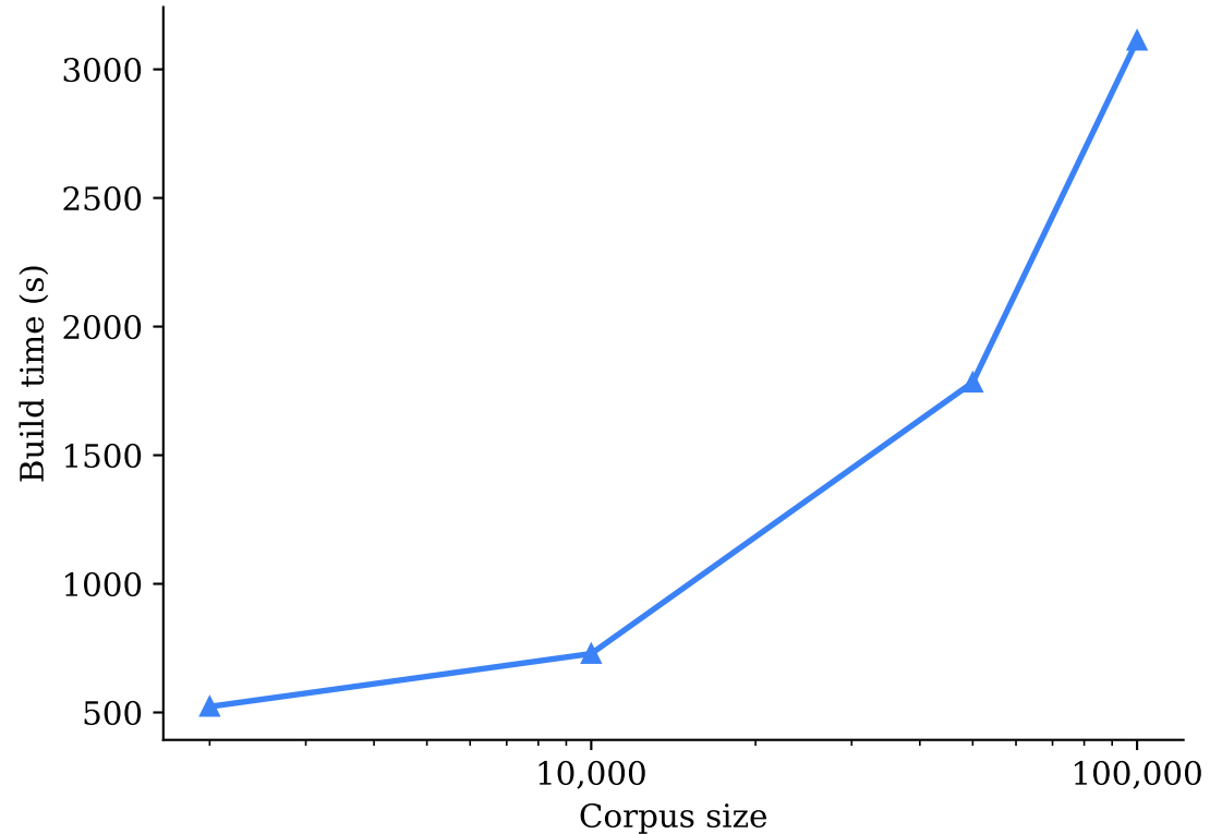
Index Build Time vs Scale
