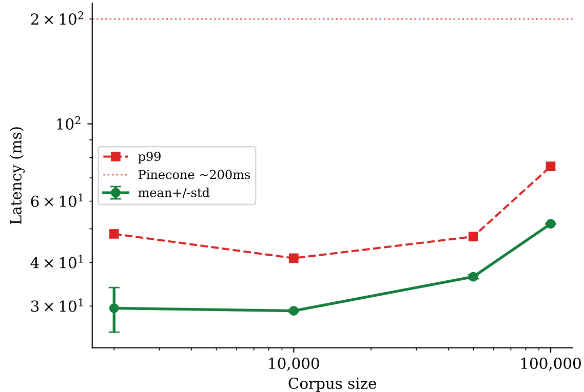
Query Latency vs Scale
