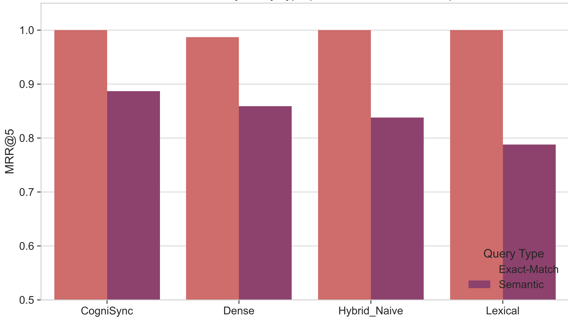
Performance by Query Type (Lexical vs Semantic Intent)
