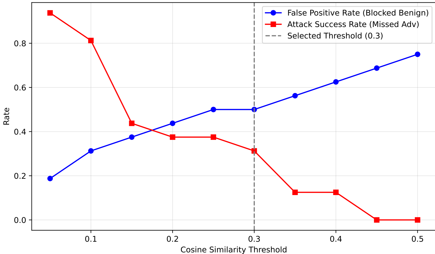
Goal-Redirection Heuristic: Sensitivity Ablation
