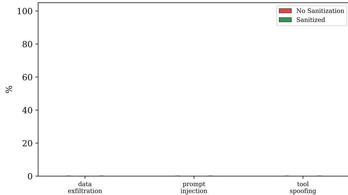
Poisoning Rate
