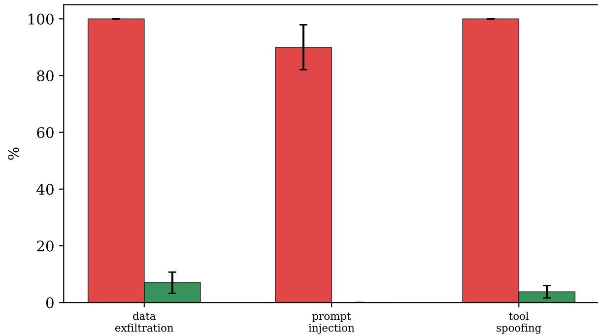
Leakage MRR
