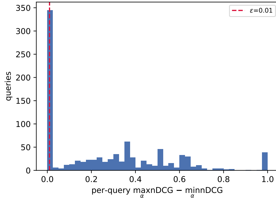
(b) 36% of queries: \alpha changes nothing
