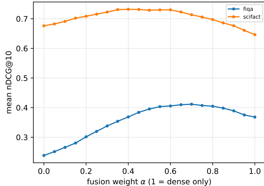
(a) nDCG is nearly flat in \alpha near the optimum
