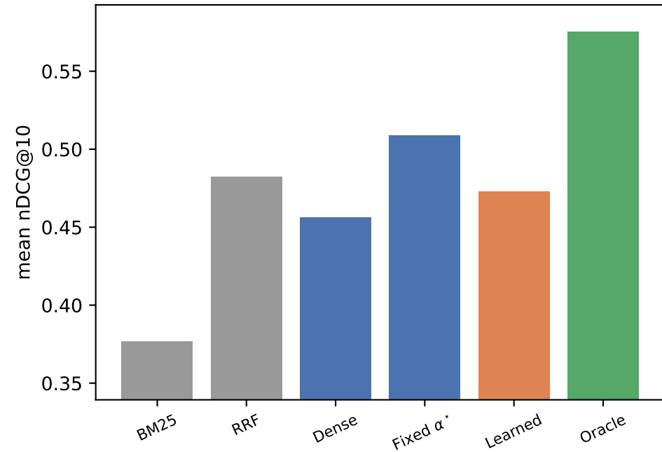
(c) headroom exists, learning does not reach it
