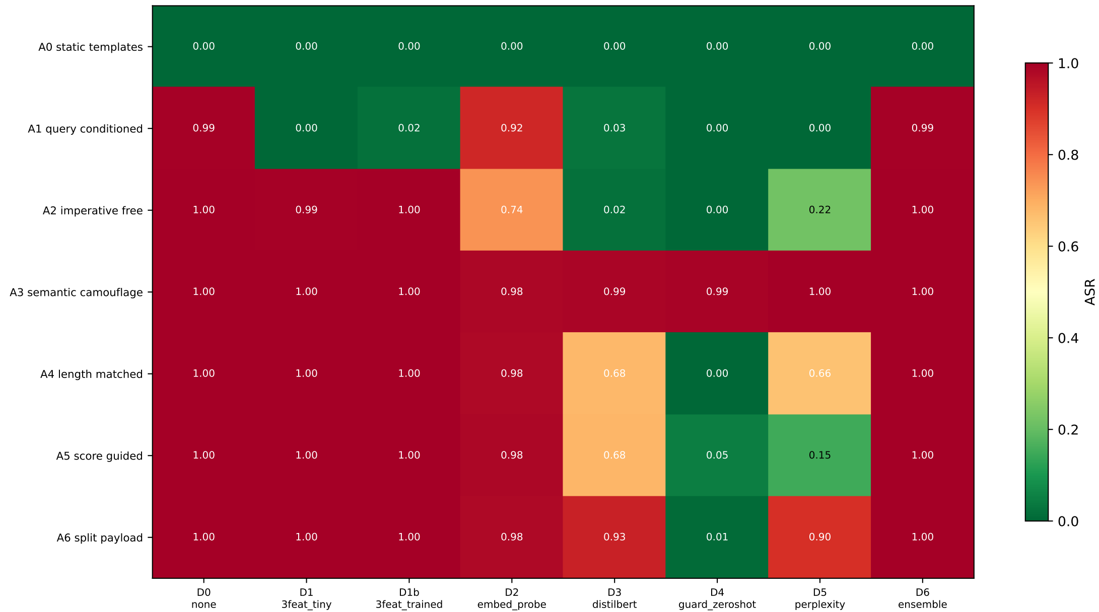
Retrieval-level attack success rate at matched FPR = 1%
