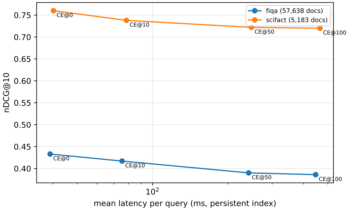
Cost/quality frontier of cross-encoder reranking
