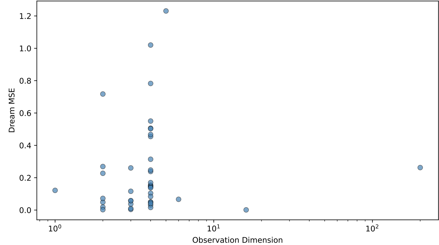
(c) Obs Dim vs Dream Quality
