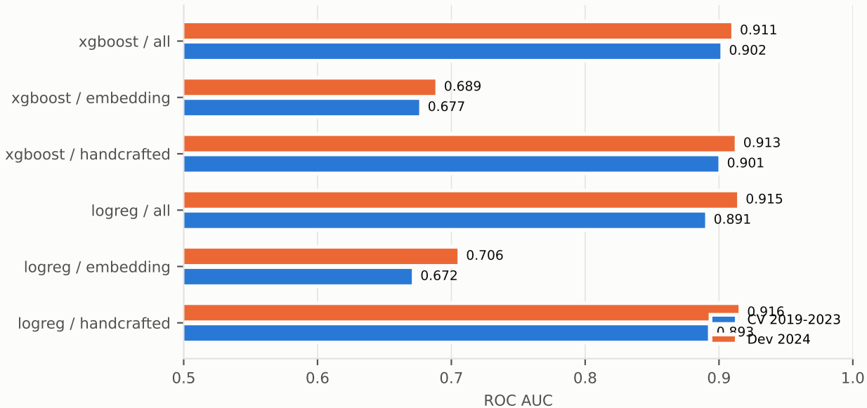
Learned verifier: classifier comparison
