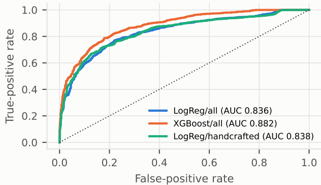
ROC on the 2025 full pool (3,040 candidates)
