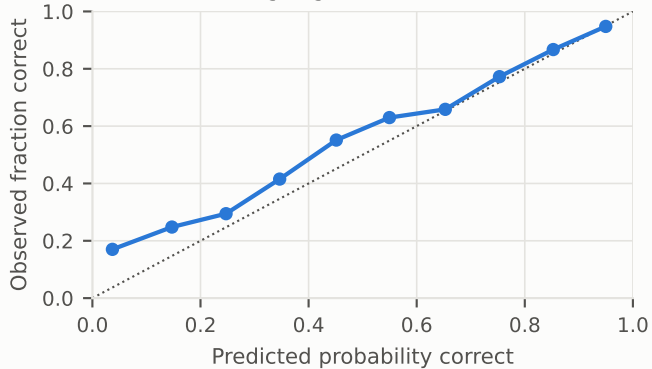
Calibration, LogReg/all (ECE 0.063)
