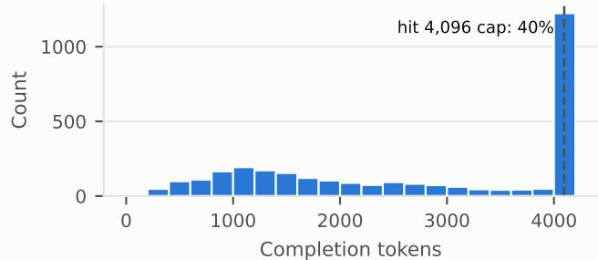
CoT length (3,040 samples)
