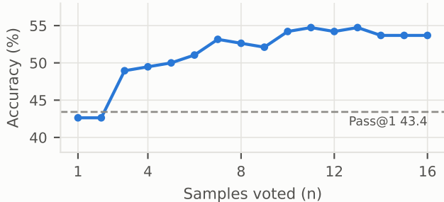
Self-consistency (majority vote), Qwen3-VL-8B
