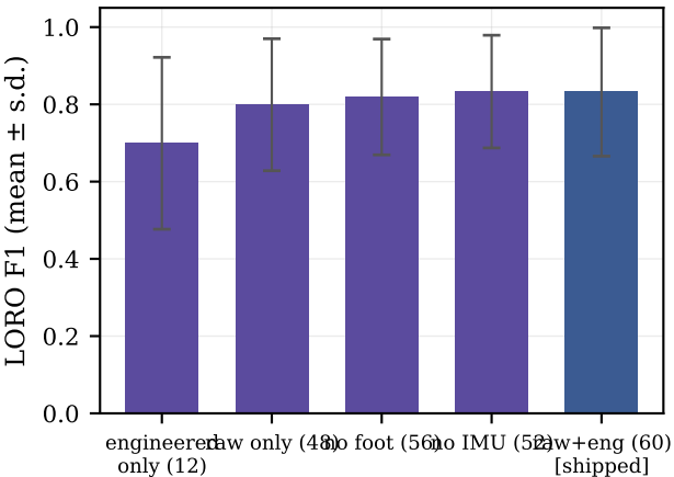
Feature-set ablation
