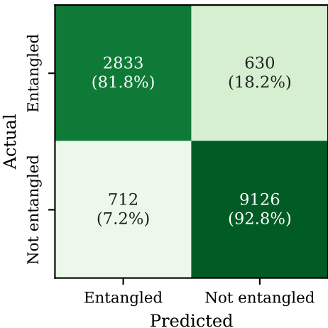
Detection confusion matrix (test split)
