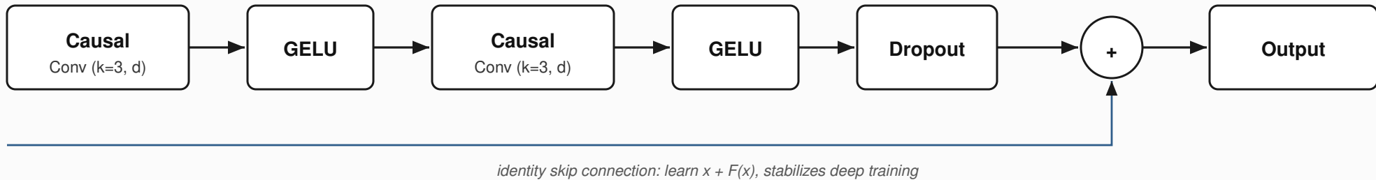
Residual TCN block (one of five; dilation d increases 1→2→4→8→16)
