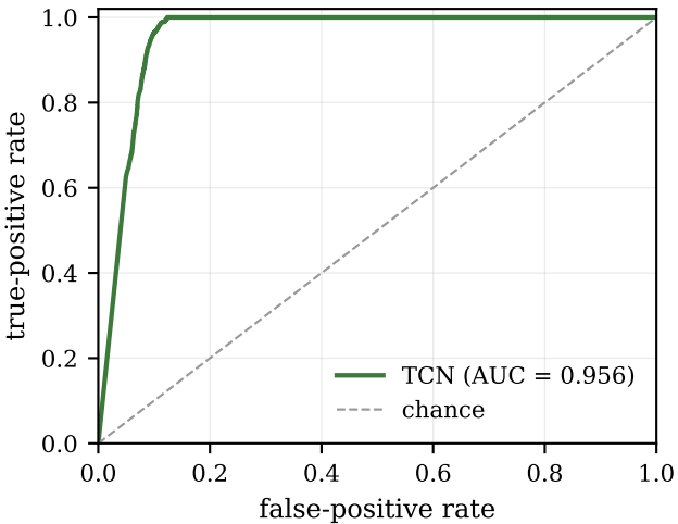
ROC (test split)
