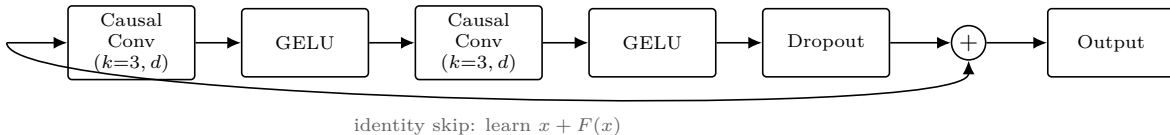
Residual TCN block (one of five; dilation d \in \{1, 2, 4, 8, 16\} )
