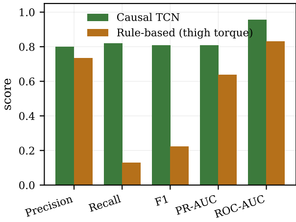
Detection: TCN vs. rule-based baseline
