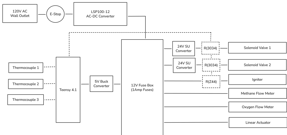
Figure 2: Electrical Wiring Diagram.
