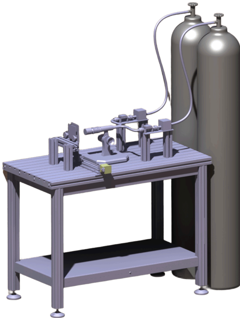
Figure 1: Prototype CAD Model.
