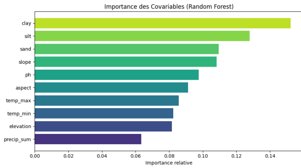
Figure 6.15 – Importance des covariables (Partie 2, Arkansas).
