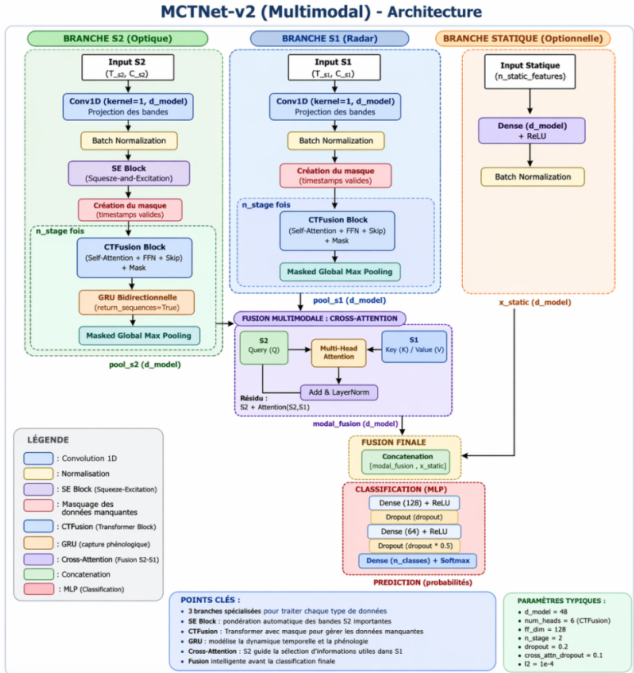
Figure 5.14 – Architecture de MCTNet-v2 (Partie 3) : double encodage temporel + attention croisée + tête bi-modale.
