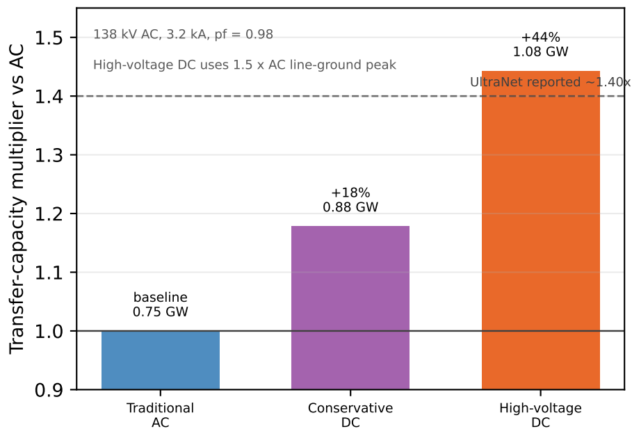
a 138 kV reference corridor
