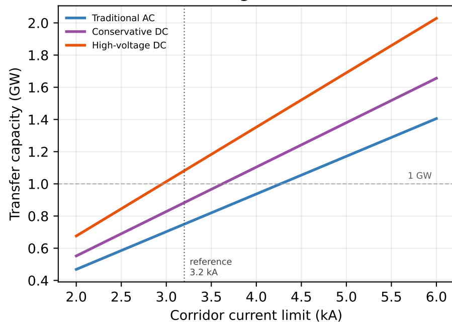
b Current-limit scaling
