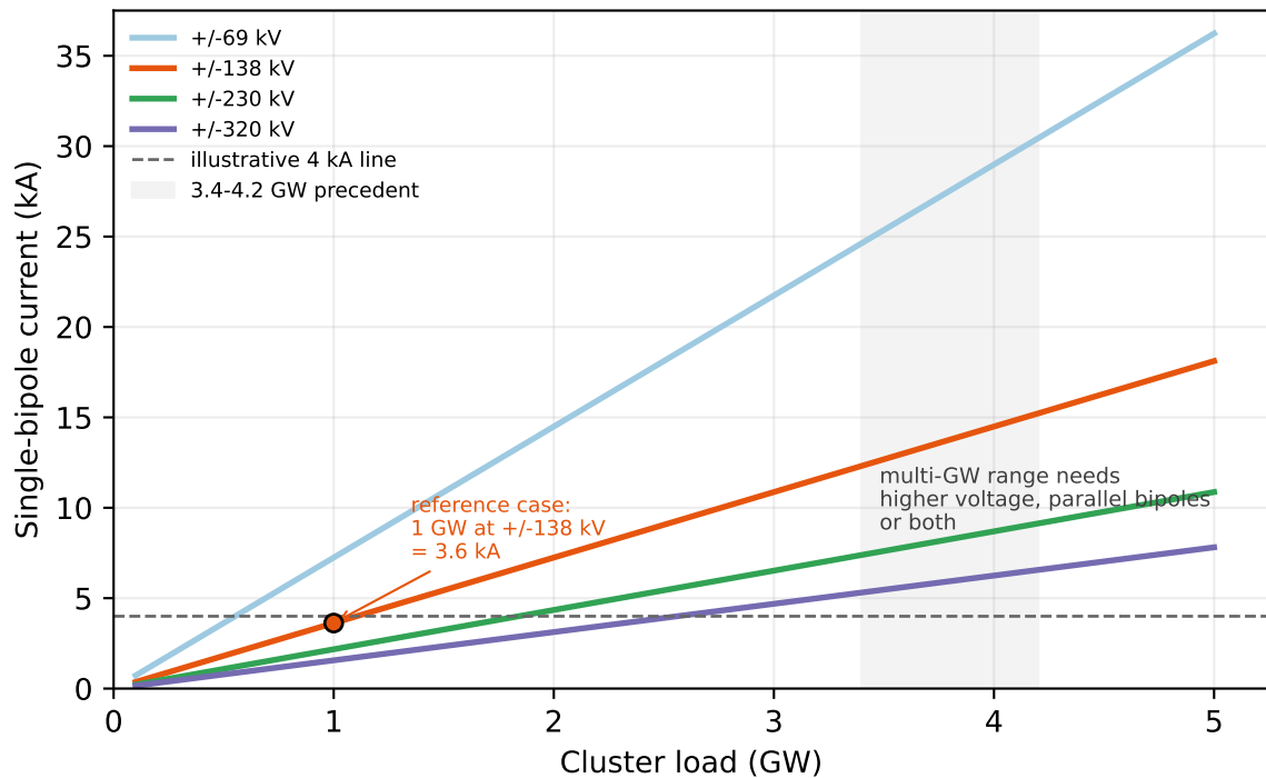
b Voltage envelope
