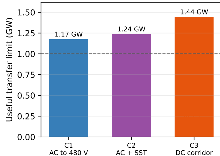
a Transfer capacity
