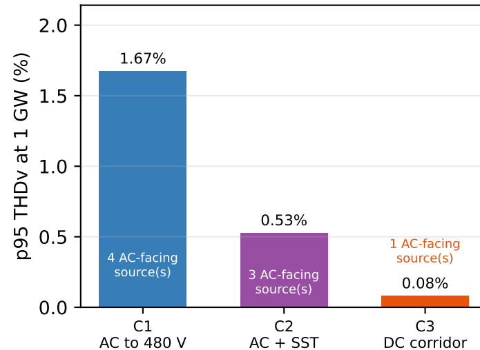
b Harmonic ownership
