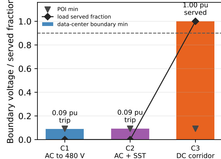
c Voltage ride-through
