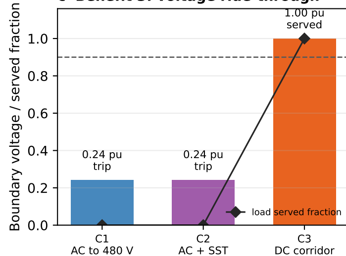
c Benefit 3: voltage ride-through
