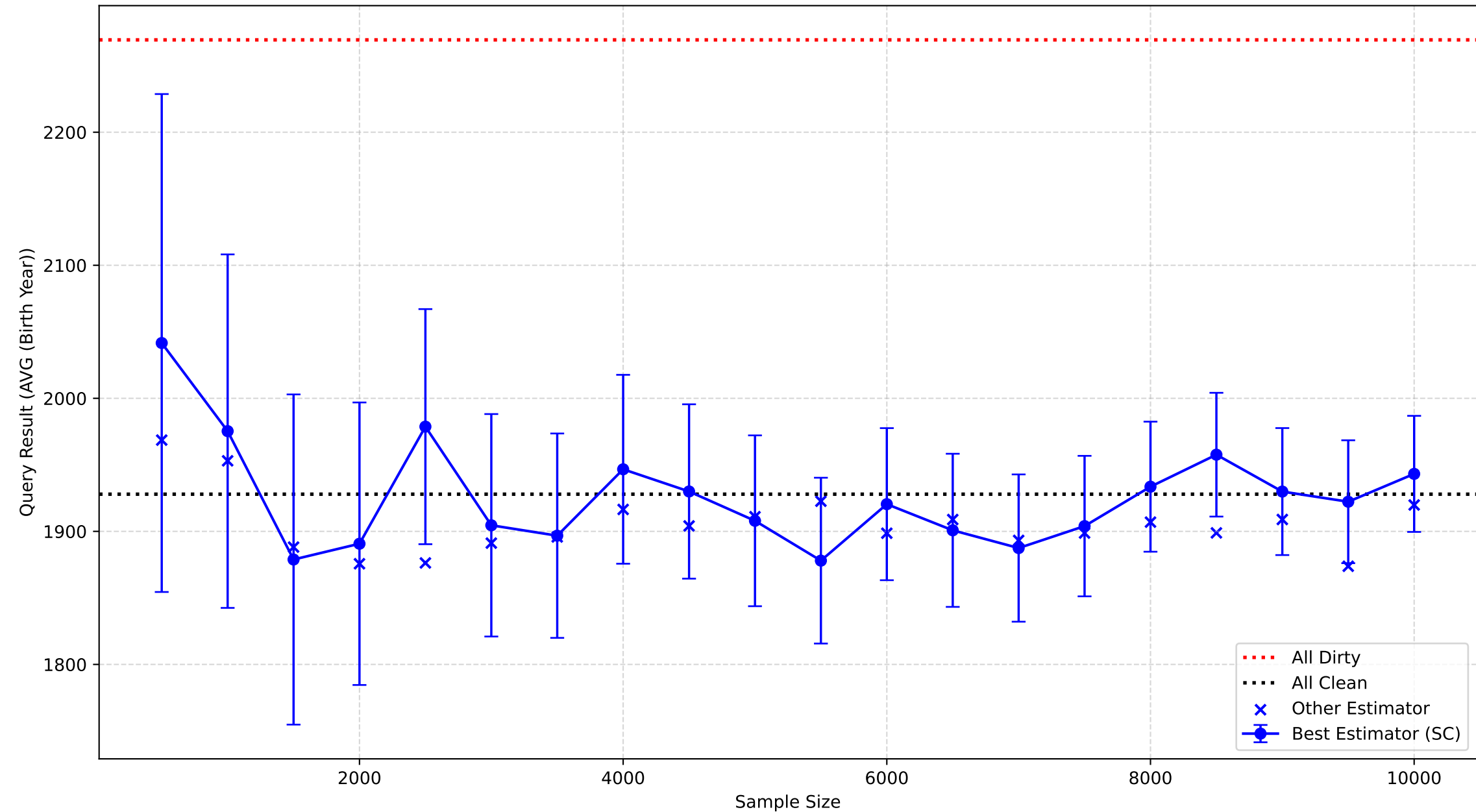
Best Estimator (RawSC or NormSC) for AVG (BIRTH YEAR)
