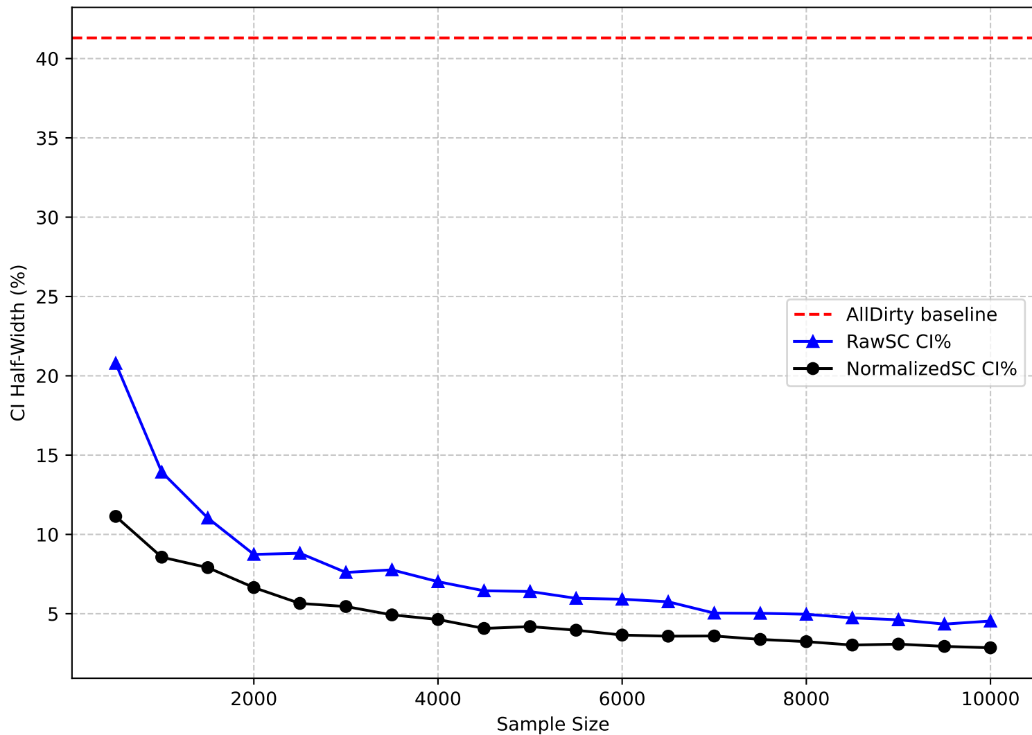
Confidence Interval % Error — SUM
