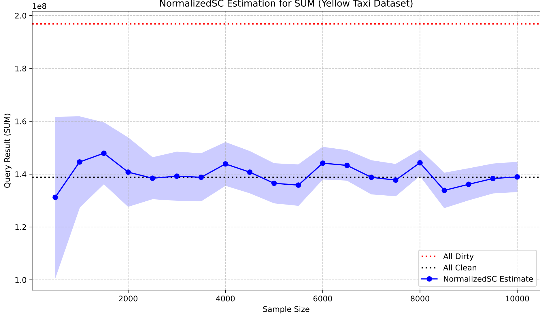
NormalizedSC Estimation for SUM (Yellow Taxi Dataset)
