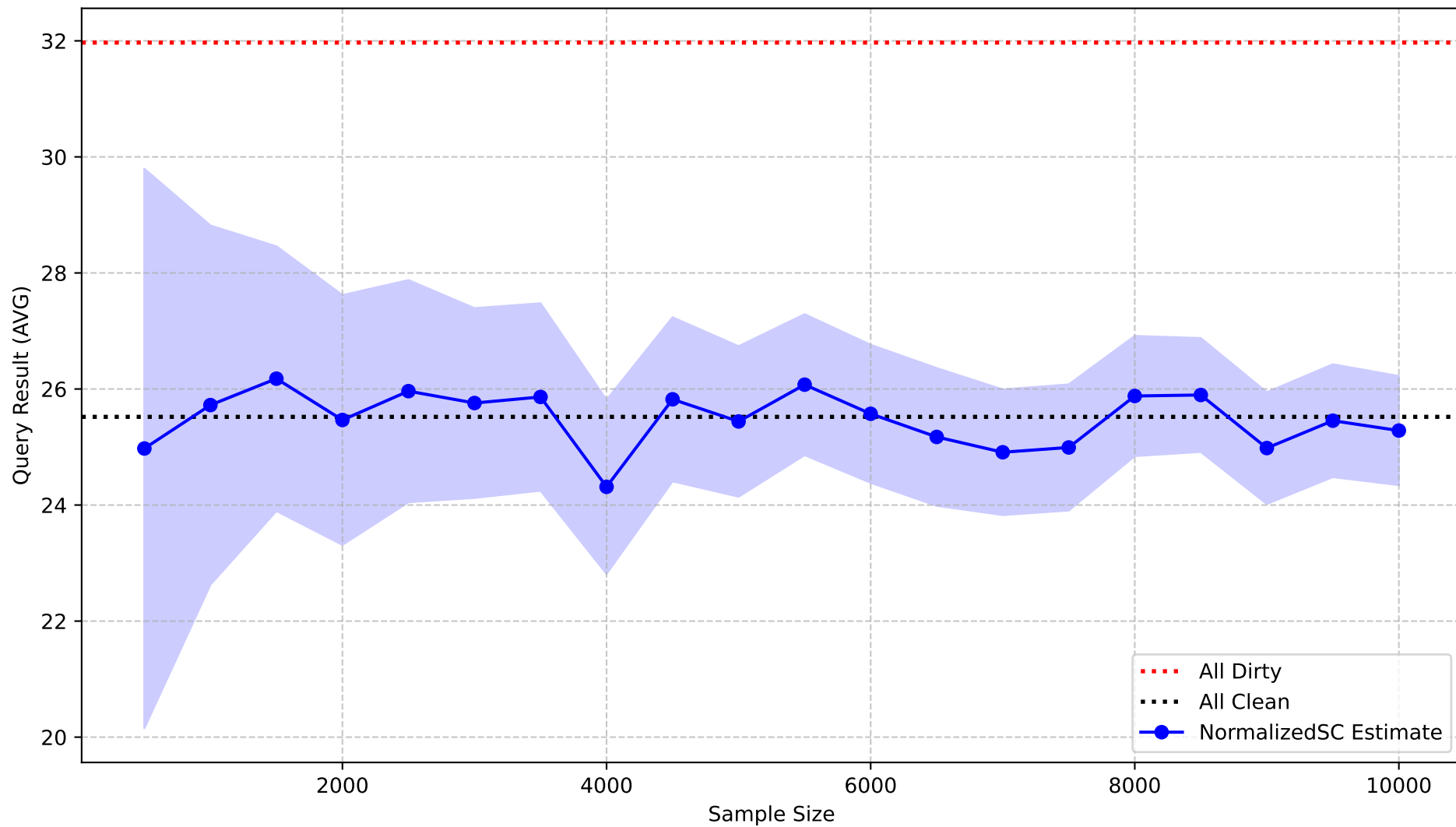
NormalizedSC Estimation for AVG (TPC-H Lineitem)
