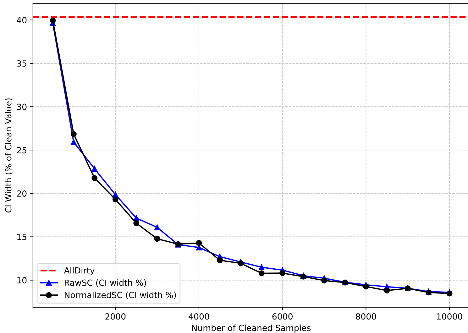
Confidence-Interval Error for SUM
