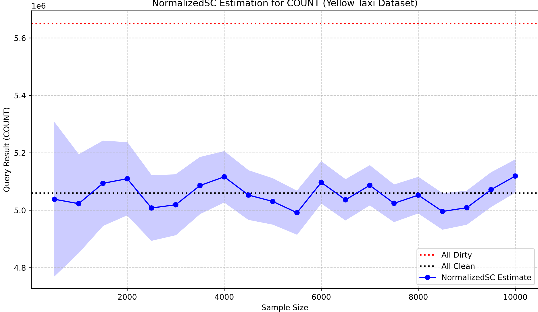
NormalizedSC Estimation for COUNT (Yellow Taxi Dataset)
