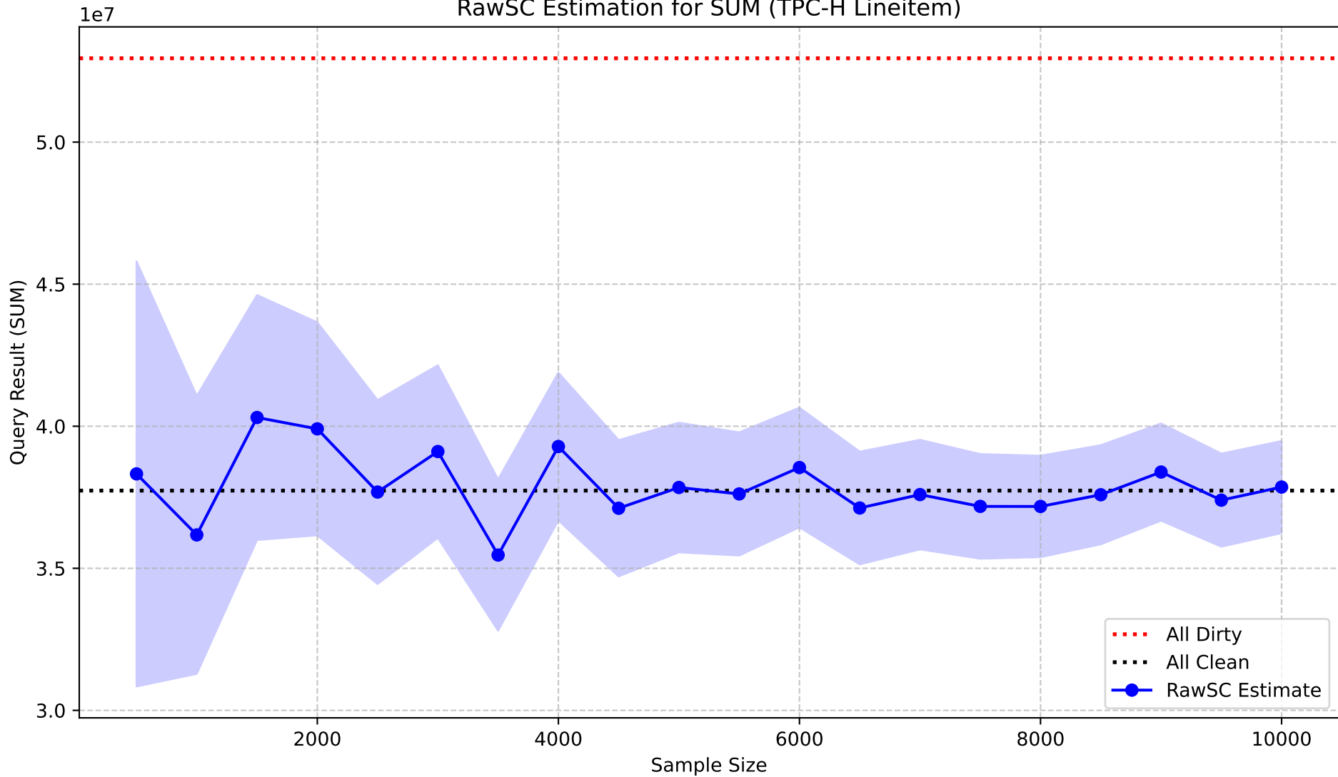
RawSC Estimation for SUM (TPC-H Lineitem)
