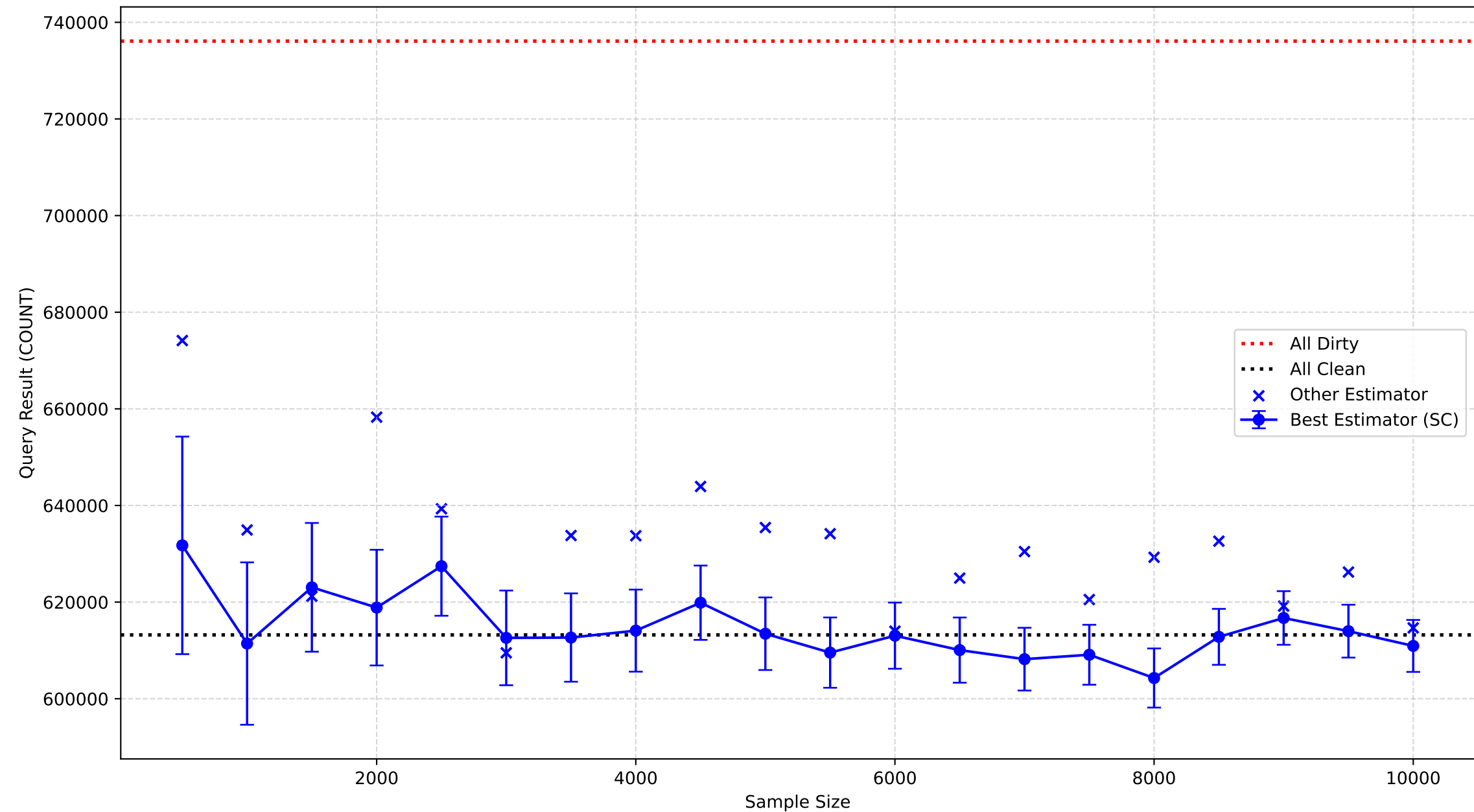
Best Estimator (RawSC or NormSC) for COUNT
