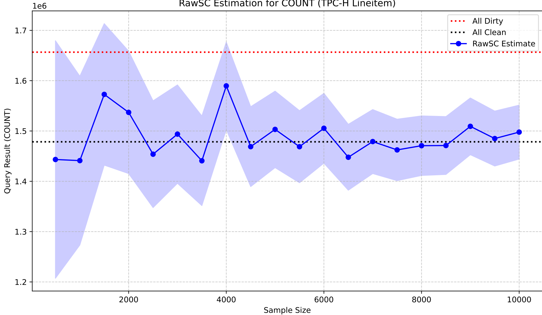
RawSC Estimation for COUNT (TPC-H Lineitem)
