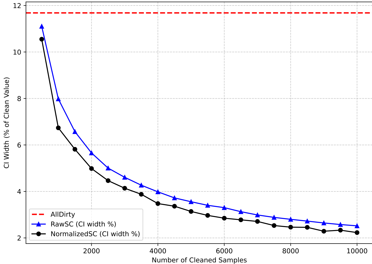
Confidence-Interval Error for COUNT (Yellow Taxi)
