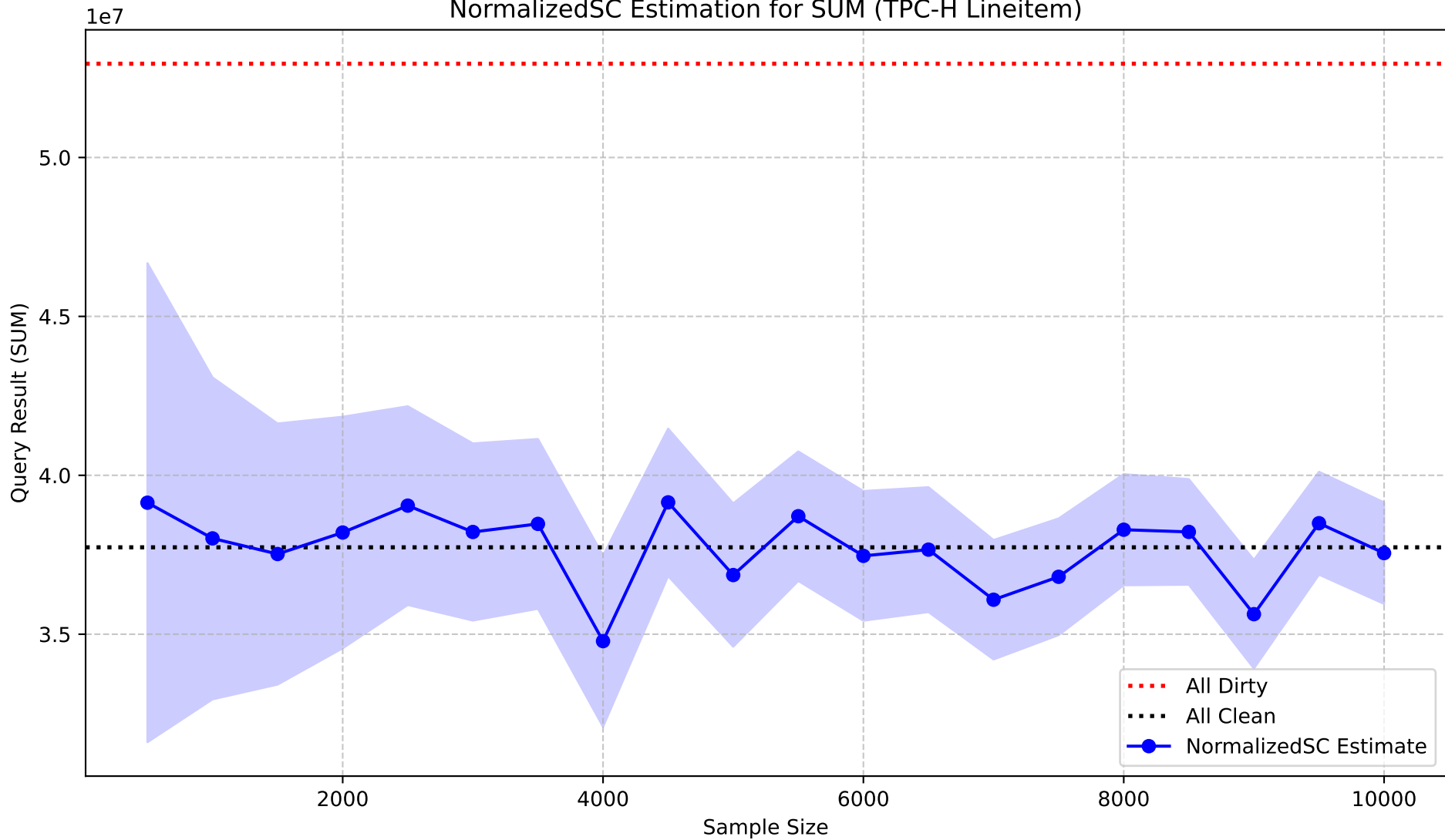
NormalizedSC Estimation for SUM (TPC-H Lineitem)
