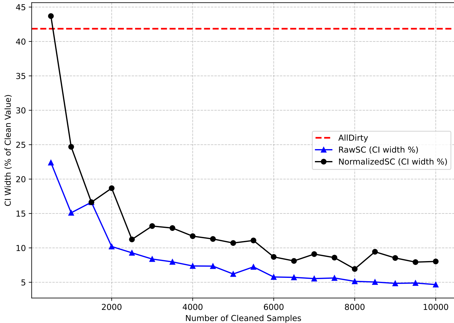
Confidence-Interval Error for SUM (Yellow Taxi)
