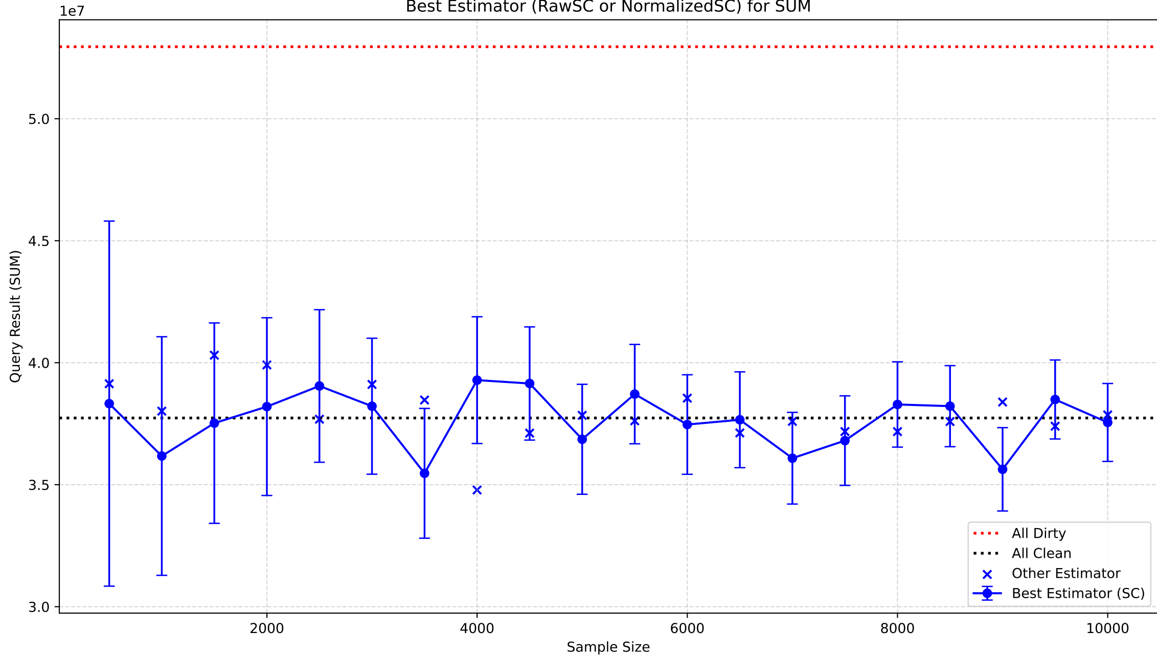
Best Estimator (RawSC or NormalizedSC) for SUM
