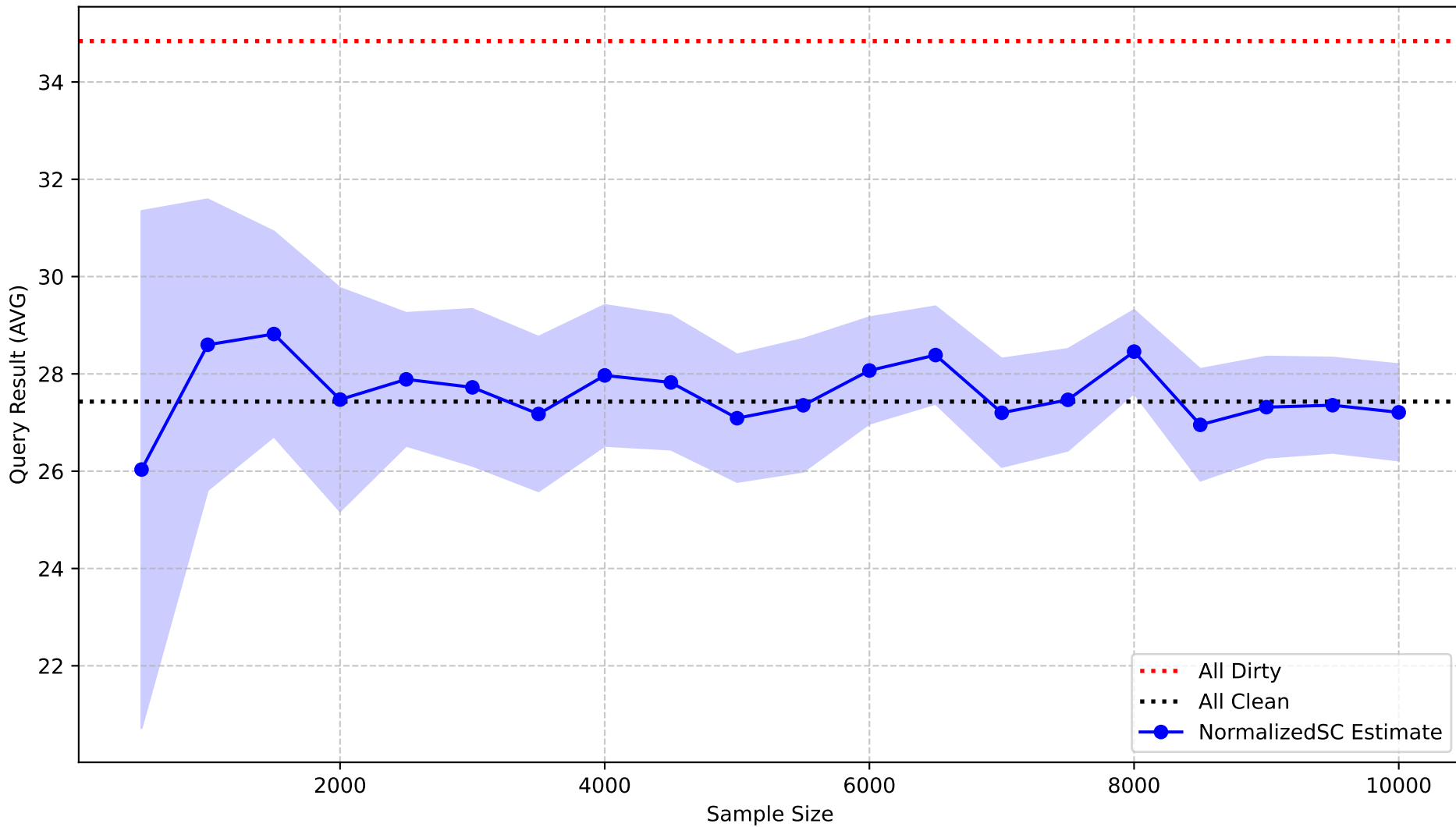
NormalizedSC Estimation for AVG (Yellow Taxi Dataset)
