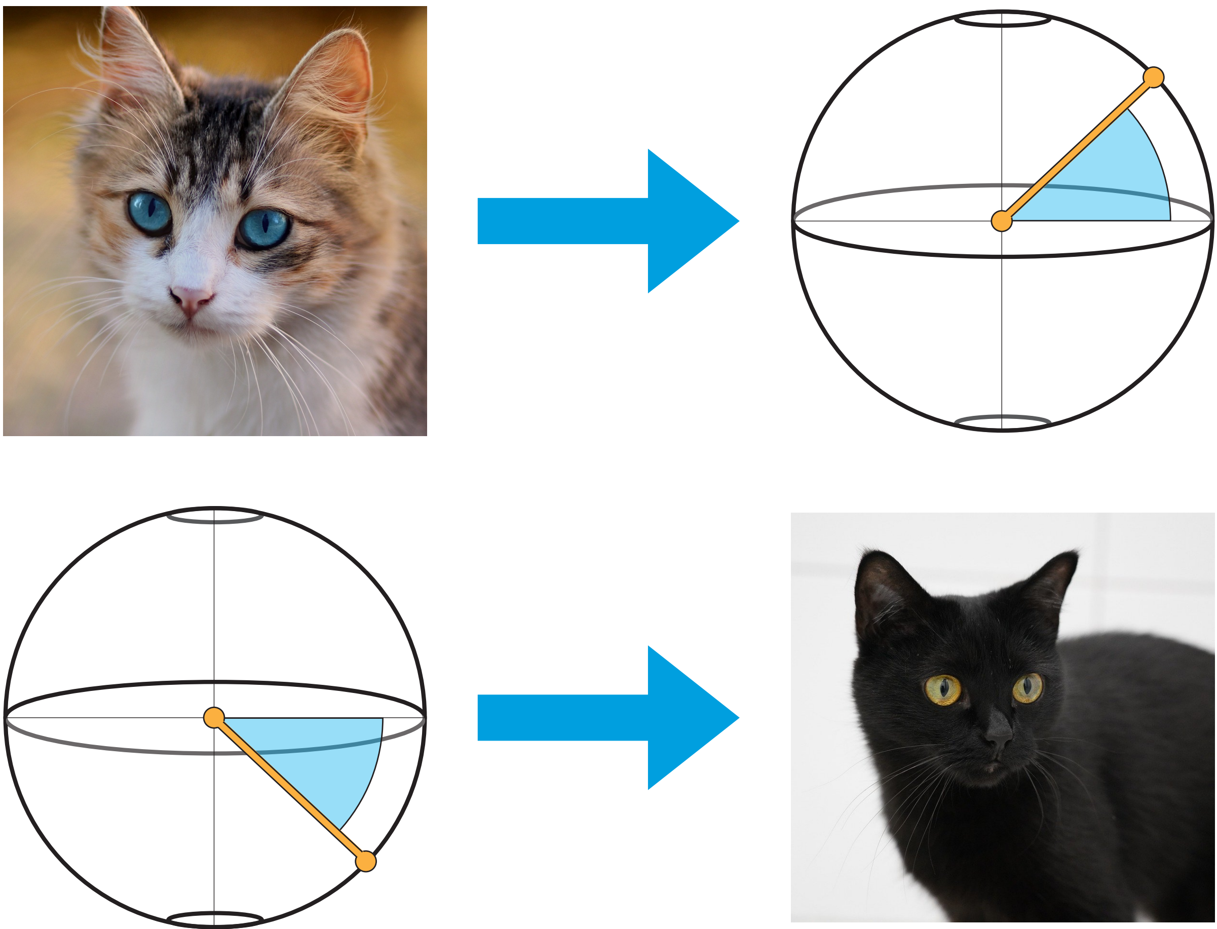
Figure 2: A cat can be encoded into a Bloch sphere and viceversa
