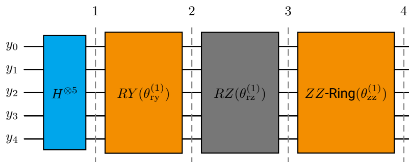
linhead
