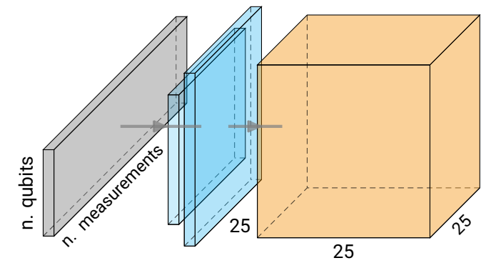
Convolution
