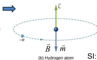
(b) Hydrogen atom
