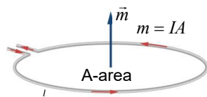
(a) Current-carrying loop
