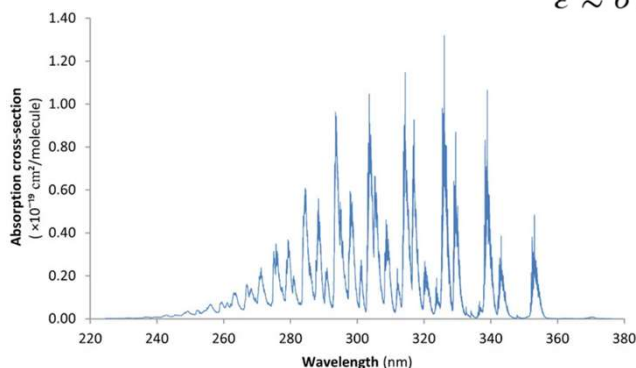
Formaldehyde absorption spectrum in the UV range, re-plotted from the data of Meller et al [30]. Peaks are not fully resolved at the resolution of this spectrum (0.01 nm).
