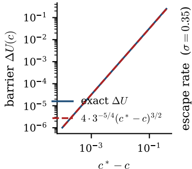
(c) 3/2 barrier scaling
