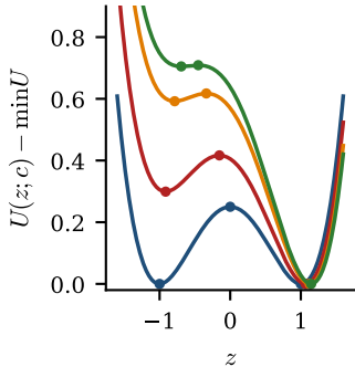
(a) tilted double well
