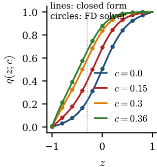
(b) committor, \sigma = 0.5
