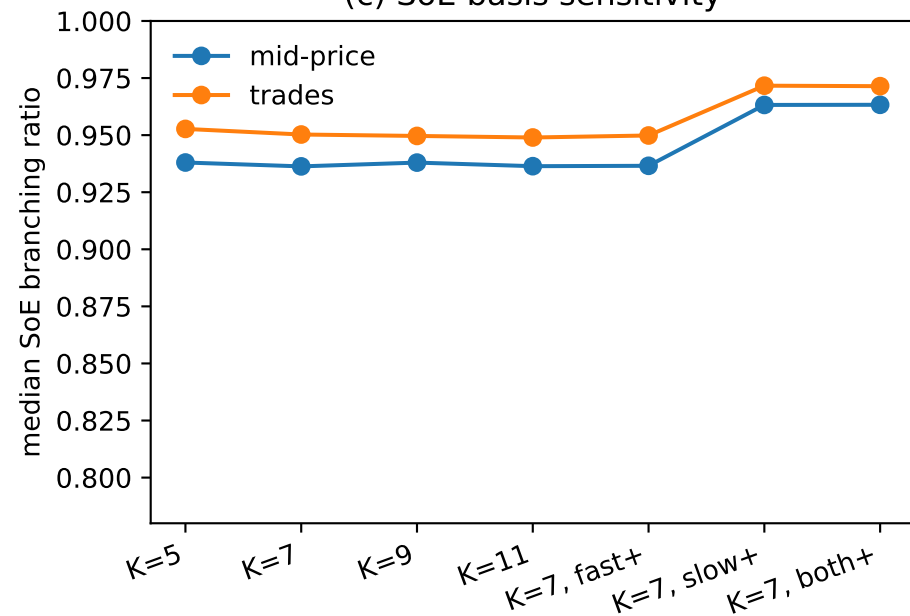
(c) SoE basis sensitivity
