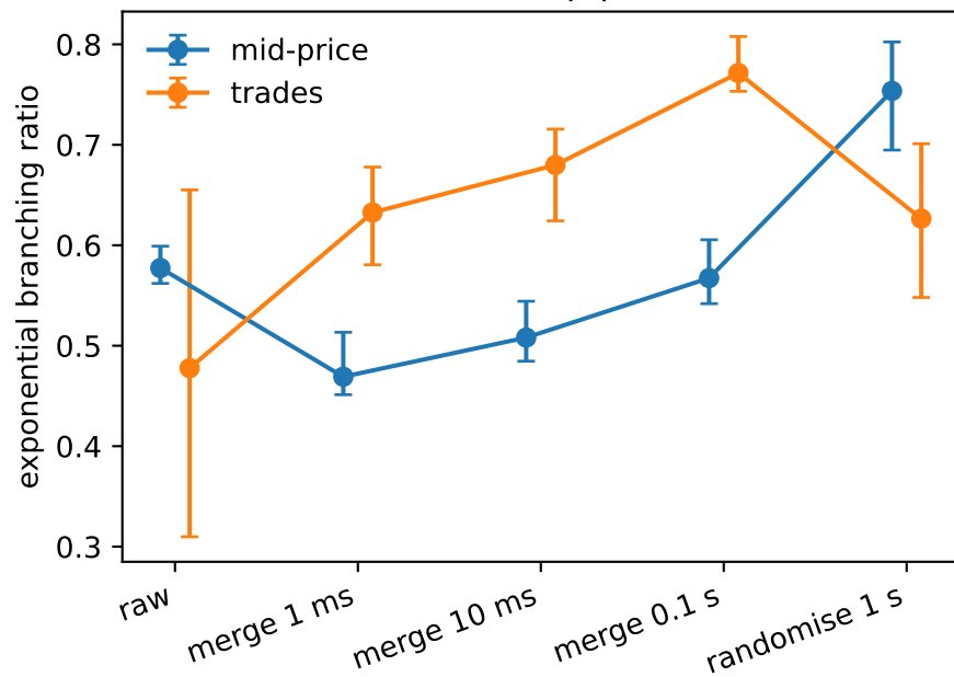
(c) SoE basis sensitivity
