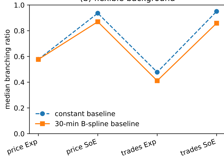
(b) flexible background
