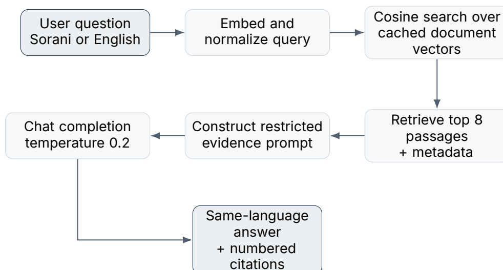
Figure 6: Grounded question-answering flow. The instruction requires the model to use only retrieved passages and to state when evidence is insufficient.
