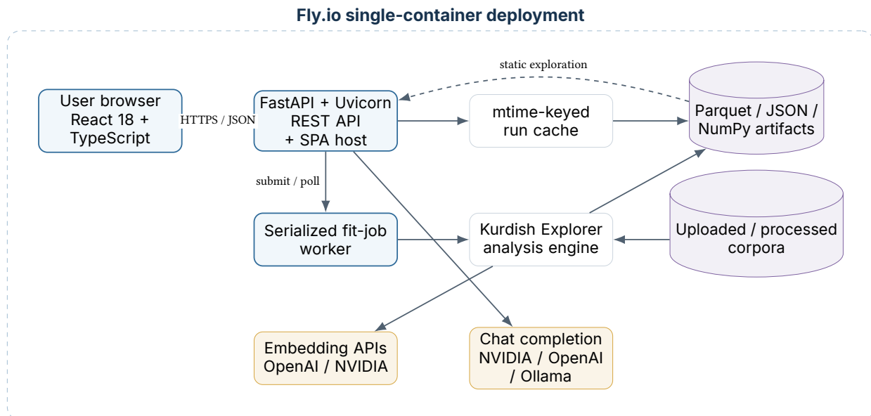
Figure 4: Production component architecture. Expensive fitting uses a serialized worker; ordinary browsing reads immutable run artifacts through the cache.
