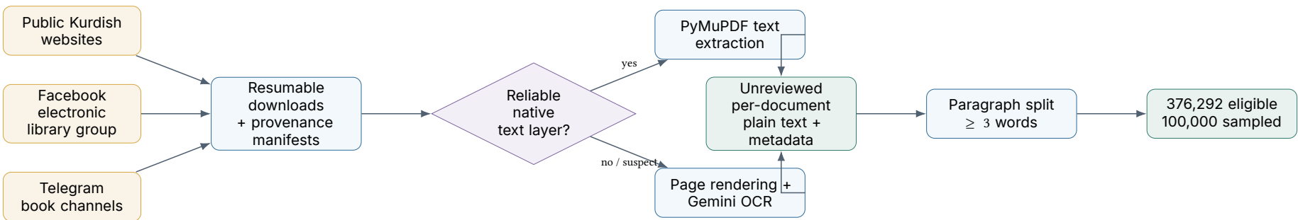
Figure 6: Verified corpus provenance from Bahdini Crawler to the deployed analytical sample. “Unreviewed” is retained as an explicit quality state.
