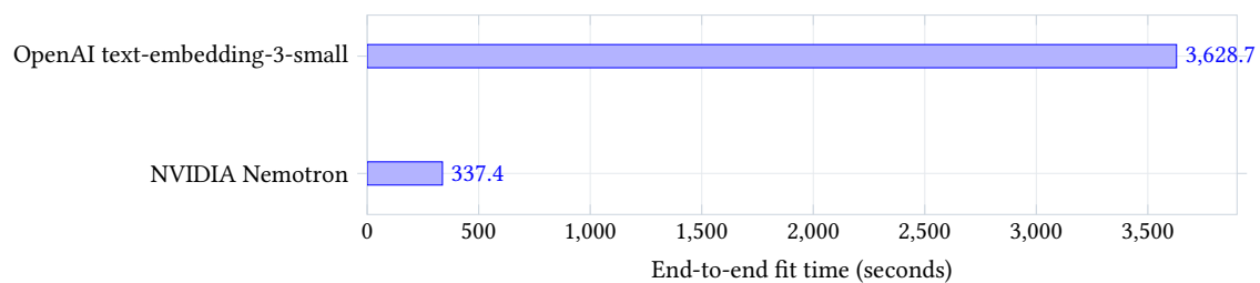
Figure 2: Measured end-to-end fitting time. NVIDIA completed the saved refit approximately 10.8 times faster.
