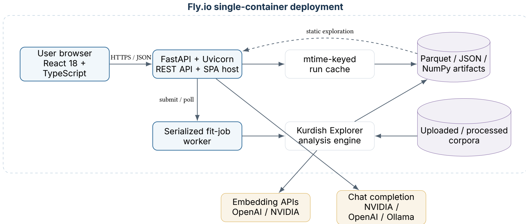
Figure 5: Production component architecture. Expensive fitting uses a serialized worker; ordinary browsing reads immutable run artifacts through the cache.
