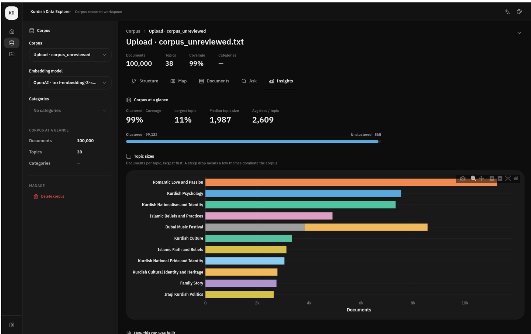
Figure 13: OpenAI run insights: topic-size distribution and exact run provenance.
