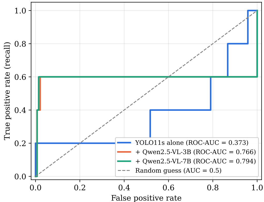
(b) ROC curve
