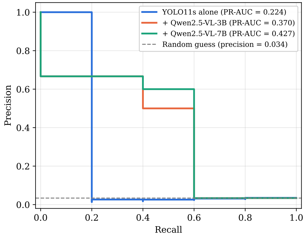
(a) Precision-recall curve
