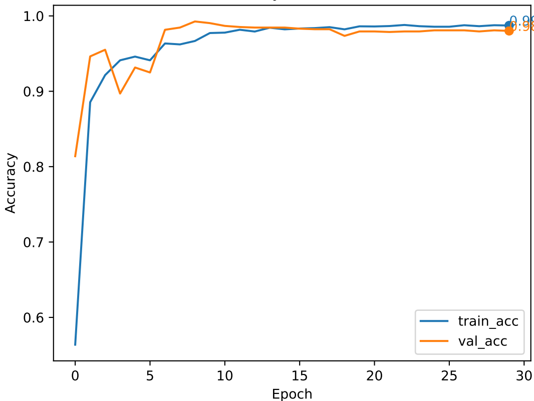
Model Accuracy - Black Box Model
