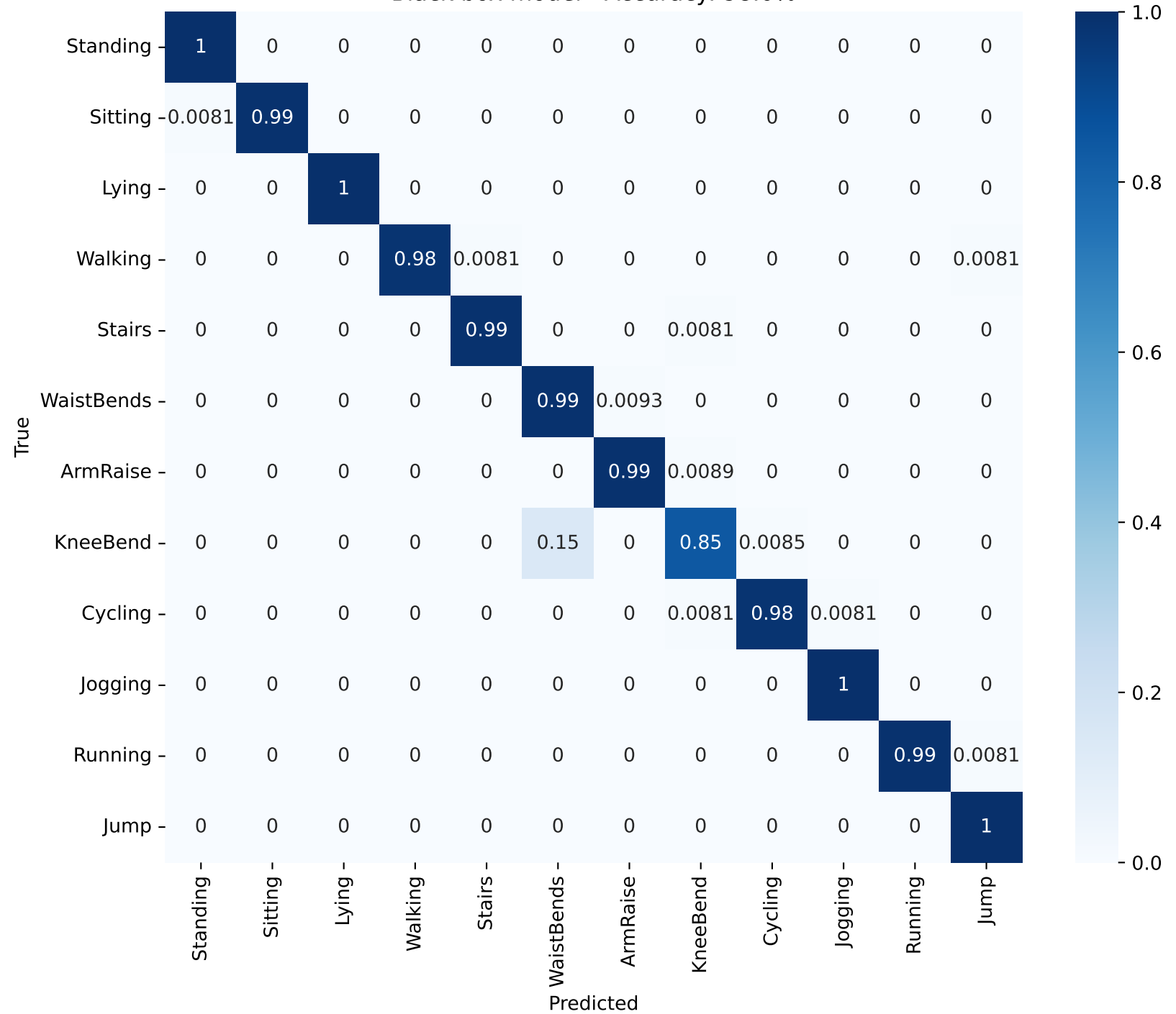
Black box model - Accuracy: 98.0%
