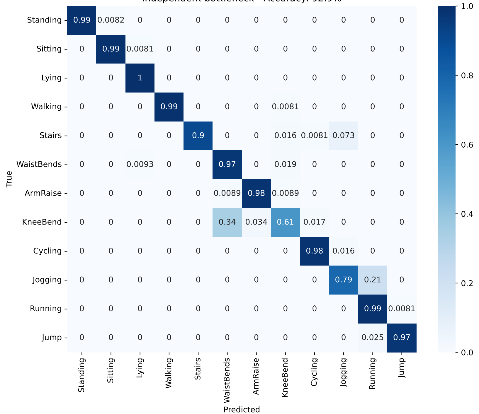
Independent bottleneck - Accuracy: 92.9%
