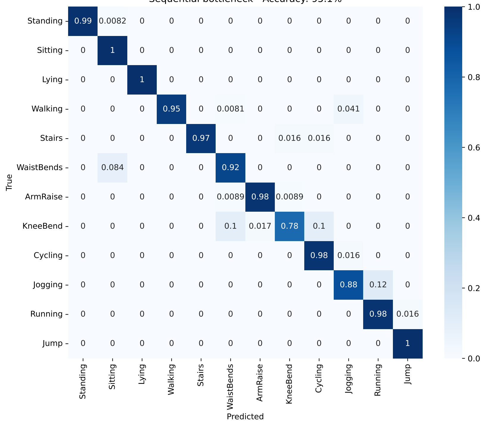
Sequential bottleneck - Accuracy: 95.1%
