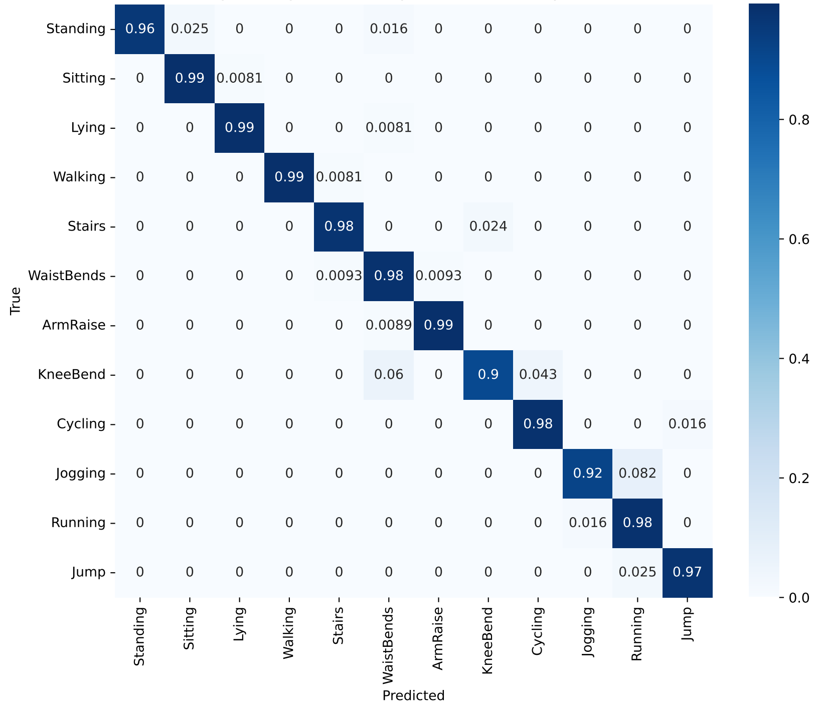
Logistic Regression (Independent) - Accuracy: 96.983
