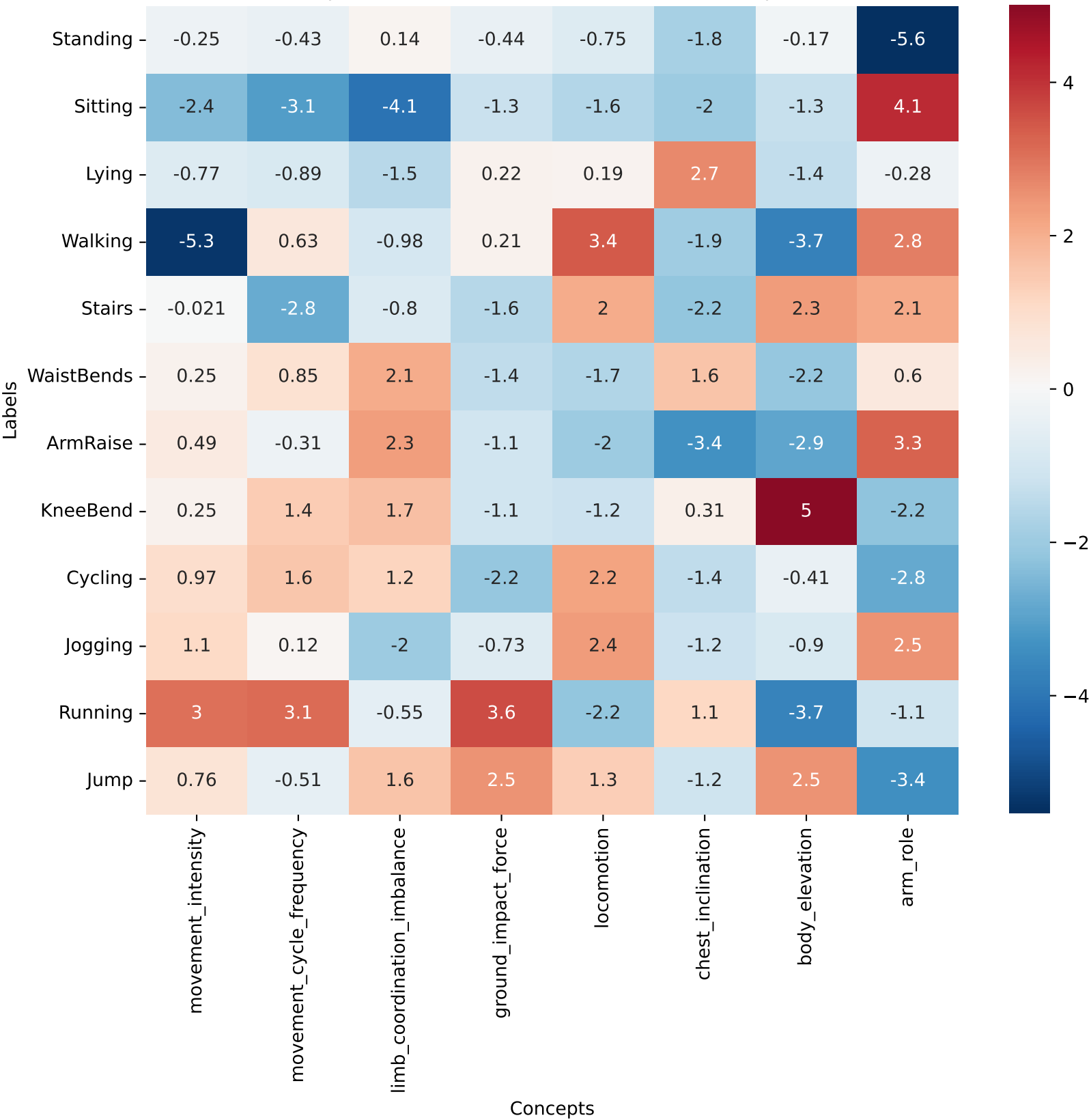
Concept-to-Label Influence (Coefficients) - Sequential
