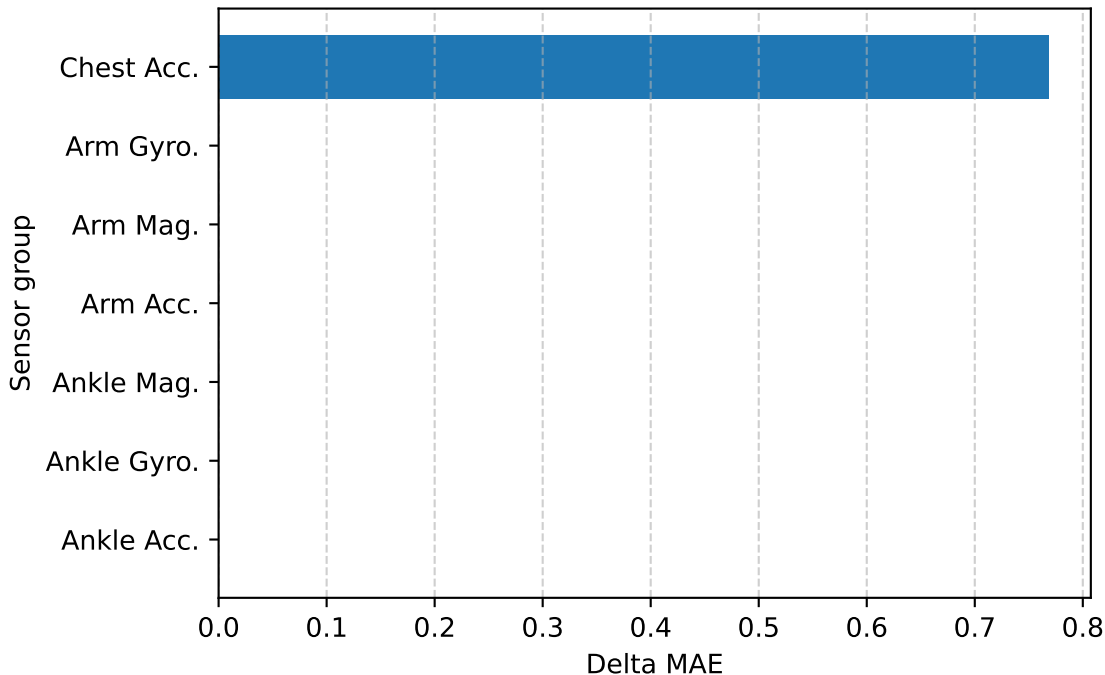
Permutation Importance by sensor group - Chest Inclination
