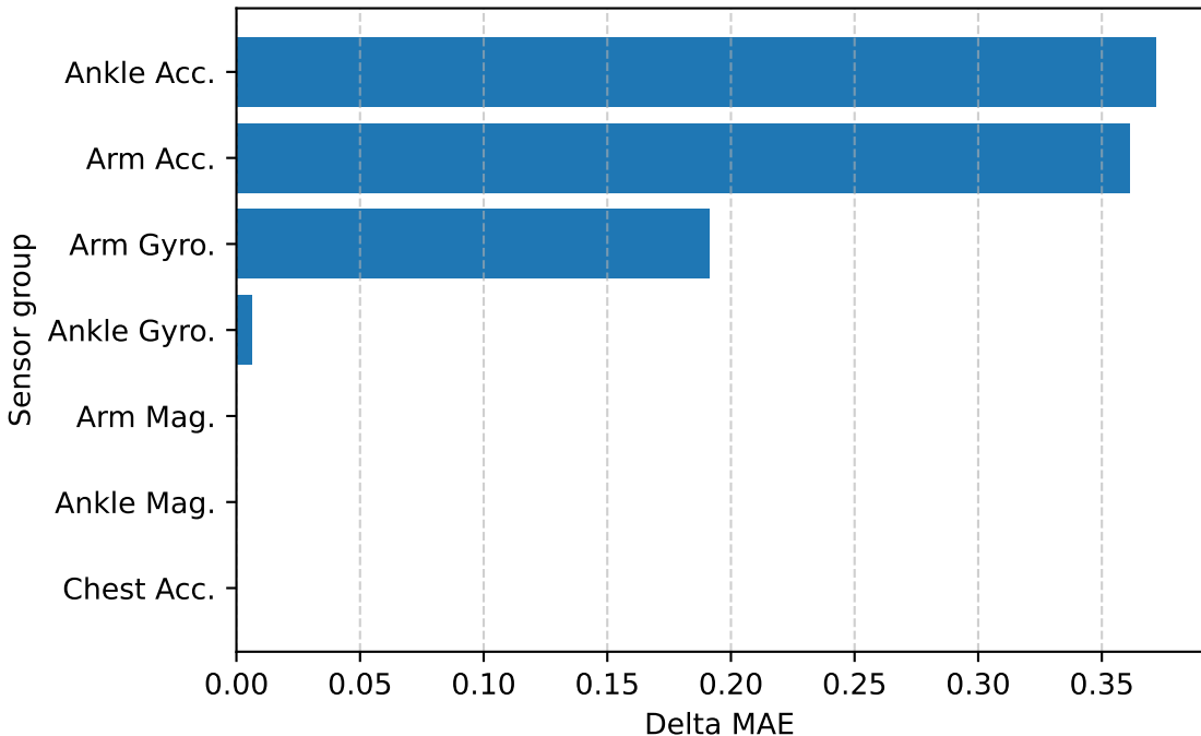
Permutation Importance by sensor group - Limb Coordination Imbalance
