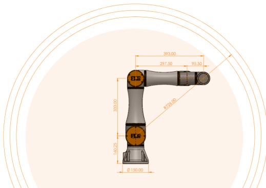
CO5 reach
