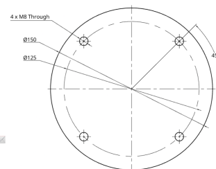
Base flange
