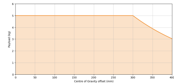
Payload curve
