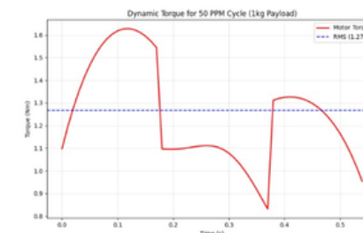
Payload curve
