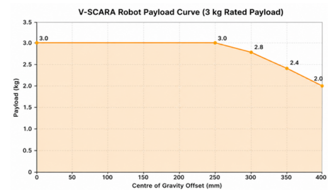
Payload curve
