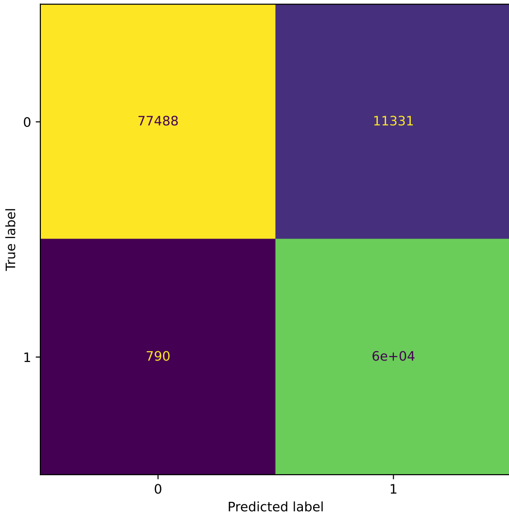
LSTM
