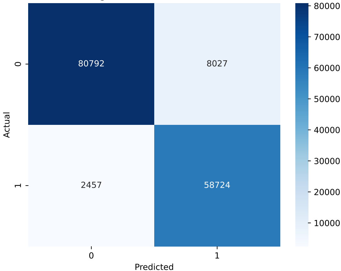
Stacking Ensemble Confusion Matrix
