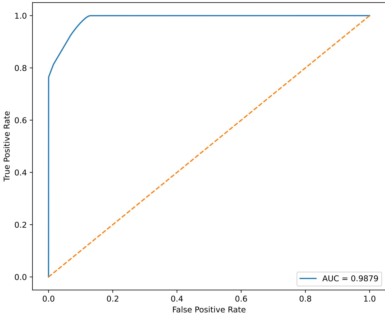
Stacking Ensemble ROC Curve
